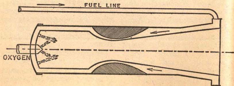
Fig. 5. Experimental American rocket motor, ca. 1946. The insert had the purpose of causing an especially fast fuel flow in the area of the nozzle's smallest diameter where the danger of a burn-through is greatest.
