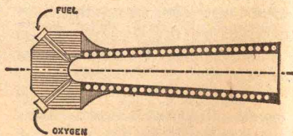
Fig. 3. Sketch for a rocket motor dated June 5, 1934. At that time Saenger evidently had not yet realized the need for a constriction in the nozzle.
