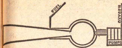
Fig. 4. Design for a rocket motor as published in the special issue of Flight . The fuel was to go directly into the cooling jacket from the tank and was to be sucked through it by the pumps. Then it was to be discharged into the combustion chamber under pressure. The oxygen was to be fed in under pressure directly.
